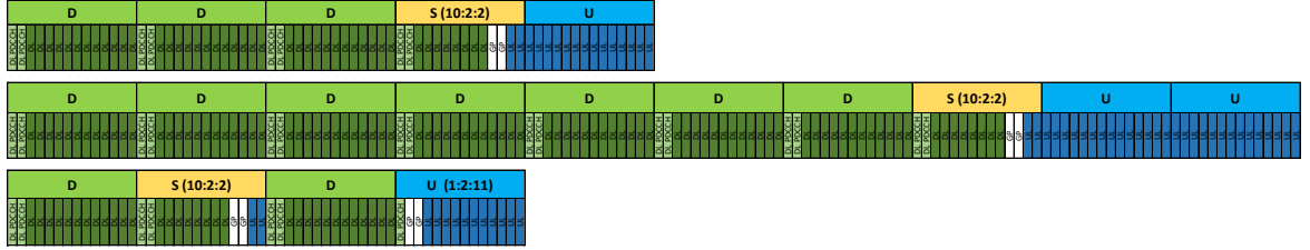
Figure 1: Three possible frame structures in 5G NR.
