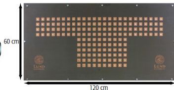
[Lund University: 160 antennas 3.5GHz]
